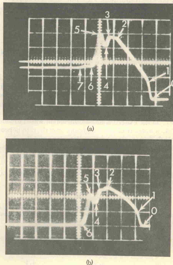
FIG. 3. (a) Oscilloscope record of a shock-wave resistance measurement of a silicon crystal. The crystal was stressed to 162 kbar. A voltage of -1.3 V was applied to the crystal. Time increases from right to left. The vertical scale is 0.5 V/div and the horizontal scale is 0.12 \mu\text{sec}/\text{div} . (b) Oscilloscope record of the induced positive voltage in a silicon crystal when stressed to 162 kbar. No voltage was applied to the crystal. Time increases from right to left. The vertical scale is 0.5 V/div and the horizontal scale is 0.12 \mu\text{sec}/\text{div} .
